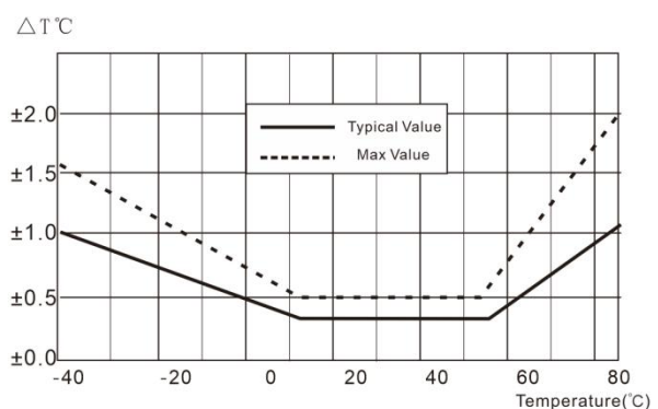
Figure 3. Typical and maximum temperature errors.
