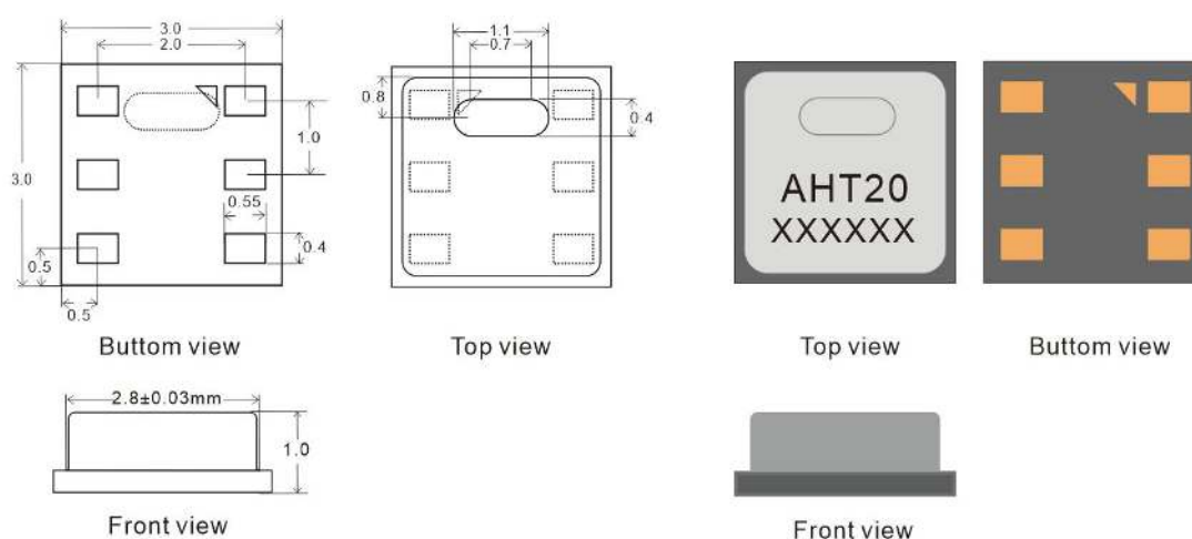
Figure 1. AHT20 Sensor Package Diagram (Unit: mm Tolerance: ±0.1 mm).
