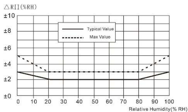
Figure 2. Typical and maximum error in relative humidity at 25°C
