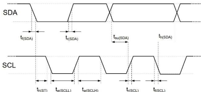
Figure 17. Timing diagram of digital input/output
