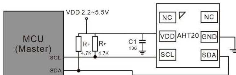
Figure 16. Typical application circuit
